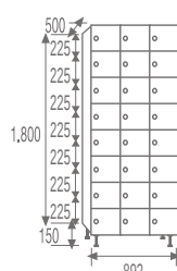
MZ-30/3 COD. 99853
