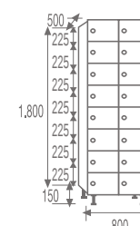
MZ-40/2 COD. 99859
