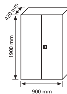
MOD. ARM01 COD. 19001
