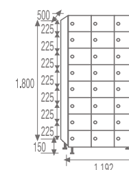
MZ-40/3 COD. 99860
