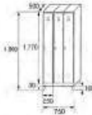
SV-25/3 COD. 42503
