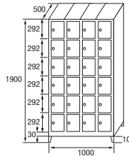
SB-25/4 COD. 42564
