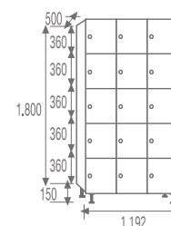
MP-40/3 COD. 99560
