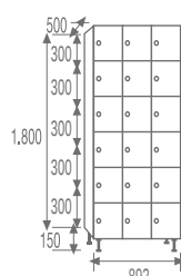
MB-30/3 COD. 99653
